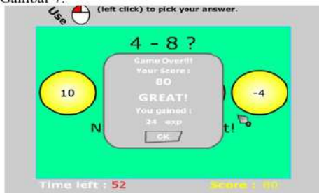
Gambar 6. Score Window
