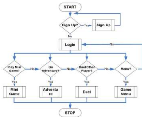
Gambar 1. Flowchart System
