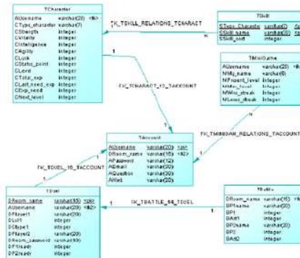
Gambar 2. ERD System
