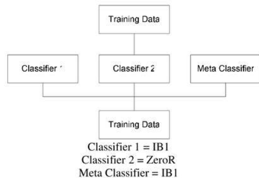
Figure 1. Design of Classifier Combination
