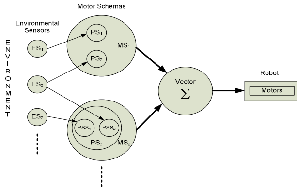
Figure 2. Motor schema method [3]
