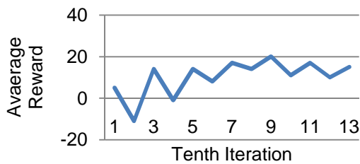
Figure 16. Average reward every tenth iteration
