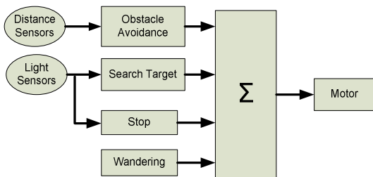
Figure 6. Robot's motor schema for autonomous navigation
