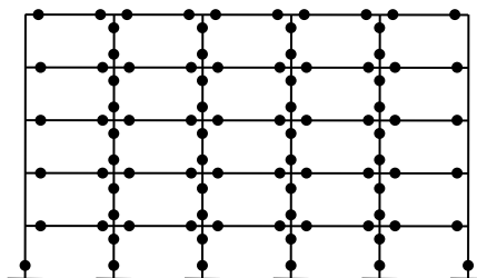
Gambar 1.4. Partial Side Sway Mechanism
