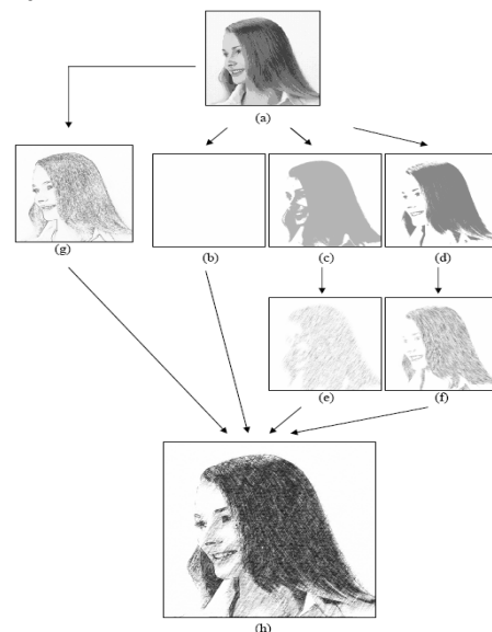
Gambar 4. Algoritma Enhanced LIC Pencil Filter Sumber: Imamiya et al (2004, p. 4)
