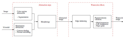
Gambar 2. Algoritma Watercolor Rendering
