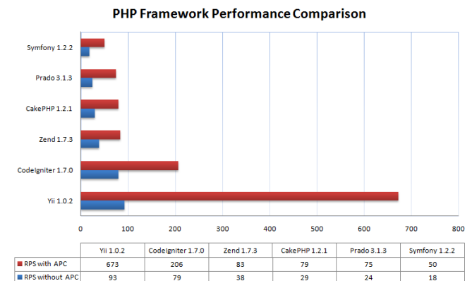
Figure 1 PHP Framework Performance Comparison [6]
