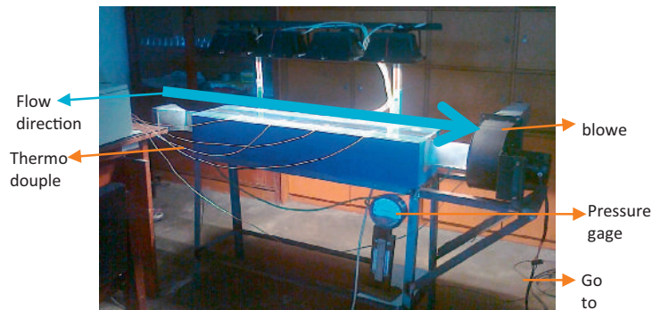
(b) Photograph of experimental set-up.
