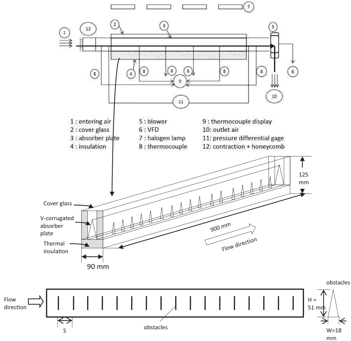
(a) Schematic of the solar collector model
