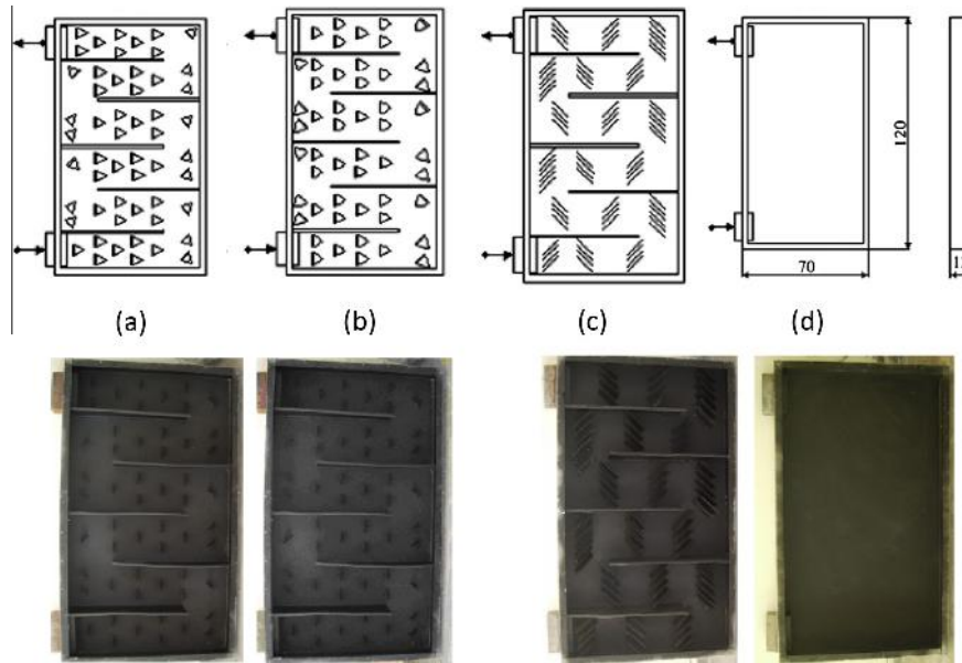
Fig. 14. Schematic views of absorber plates: (a) with triangular type obstacles, (b) with leaf type obstacles, (c) with rectangular type obstacles, and (d) without obstacles (Akpınar dan and Koçyiğit, 2010).
