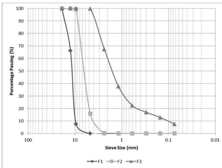
Fig 1. Sieve analysis results of tested aggregates
