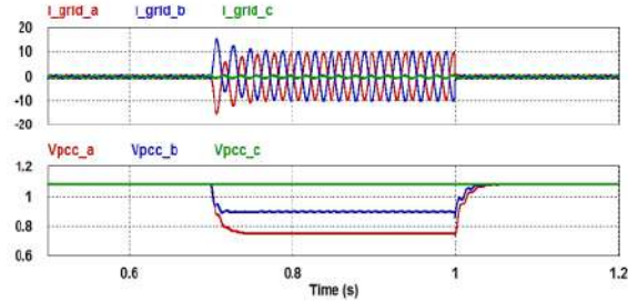
Fig. 6. A LL fault (unsymmetrical fault): Grid fault currents (top), and PCC voltages (bottom) without reactive power control.
