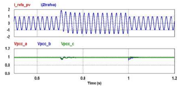
Fig. 17. With phase shift strategy: The secondary winding current is the same as the reference current (top), and the PCC voltages (bottom) for a LL fault.
