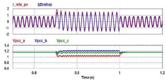
Fig. 18. Without phase shift strategy: The secondary winding current is different from the reference current (top), and the PCC is poor (bottom) for a LL fault.
