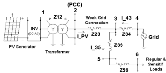
Fig. 3. A typical power system with PV installation.
