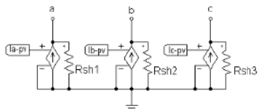
Fig. 1. A three-phase PV average model.
