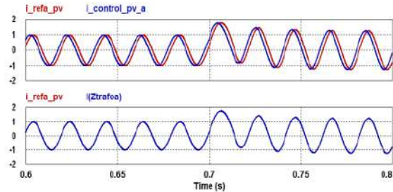
Fig. 14. A phase shift between the reference current and the controller output current (top), the secondary winding current is the same as the reference phase A.
