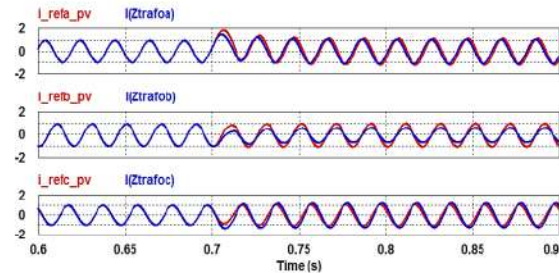
Fig. 20. Secondary winding currents are not the same as reference currents during a SLG fault.
