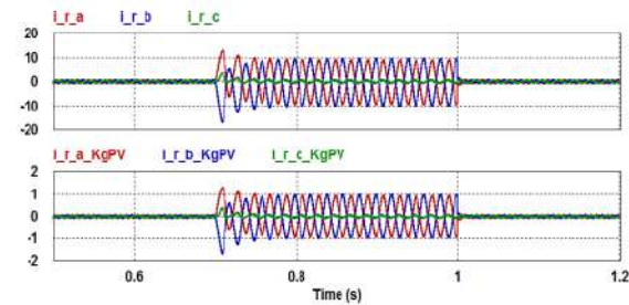
Fig. 9. A LL fault: A three-phase unbalanced reactive current (top), and a fraction of a three-phase unbalanced reactive current (bottom).
