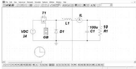
Gambar 6. PSIM: Rangkaian Buck Converter
