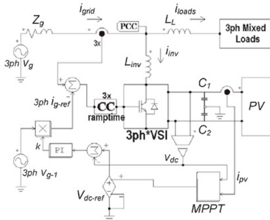
Figure 1. The proposed CC-VSI configuration
