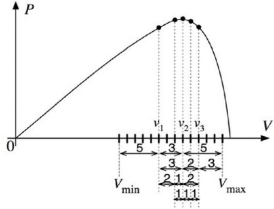
Figure 4. Searching process
