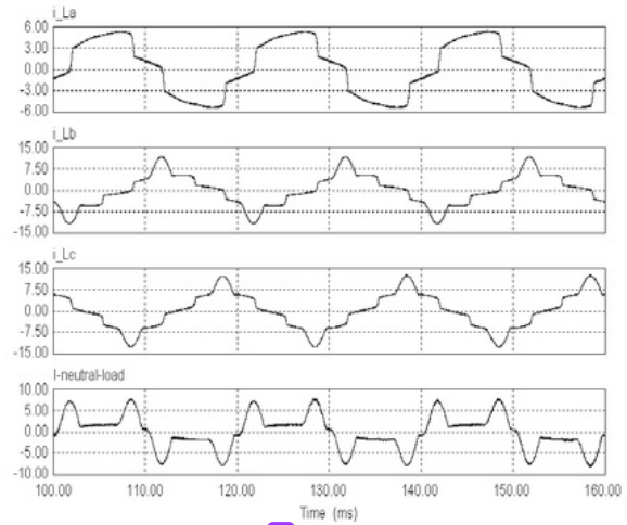
Figure 5. Mixed-load currents (phase a-b-c-neutral)
