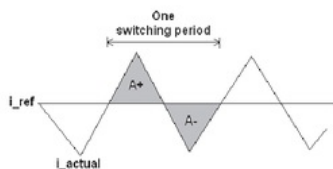
Figure 2. Zero average current error (ZACE)
