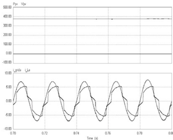
Figure 8. PV output voltage and power under zero insolation level (top); the grid and the load currents – phase A (bottom)
