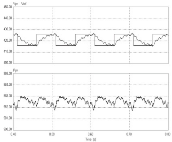
Figure 6. PV output voltage and its reference (square wave) (top); PV output power (bottom)
