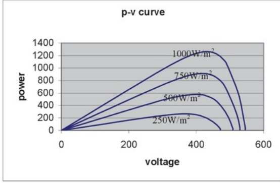
Figure 3. p - v curves of the PV array
