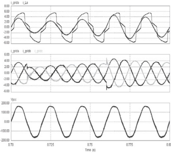
Figure 7. (top to bottom) the grid and the load currents (phase A); three-phase grid currents; the grid voltage (phase A)
