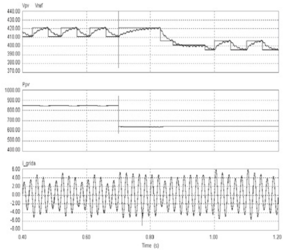
Figure 9. When the insolation is changed ( 0.7\text{kW/m}^2 to 0.55\text{kW/m}^2 ) (top to bottom): PV output voltage (and its reference); PV output power; the grid current (phase A)
