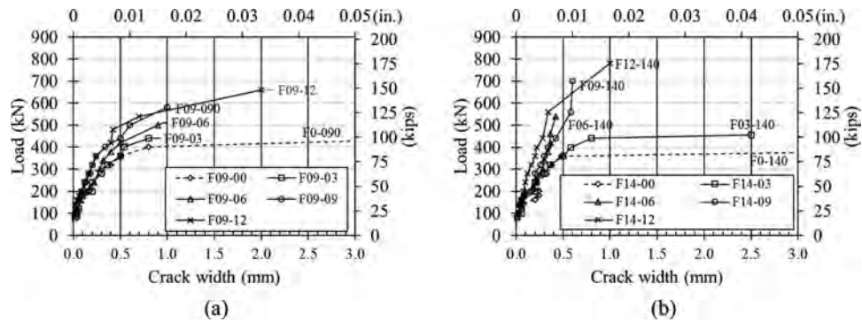
Fig. 7—Cracks widths in: (a) F09 specimens; and (b) F14 specimens.
