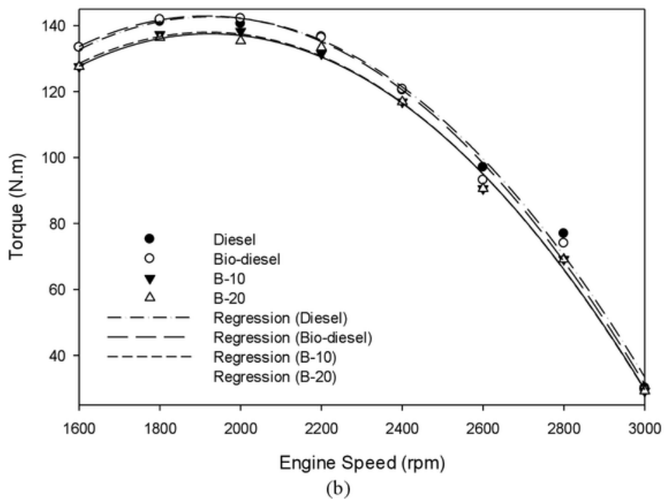
Fig. 7. Engine performance test results for various fuels in terms of (a) Brake power output of the engine and (b) Torque of the engine.
