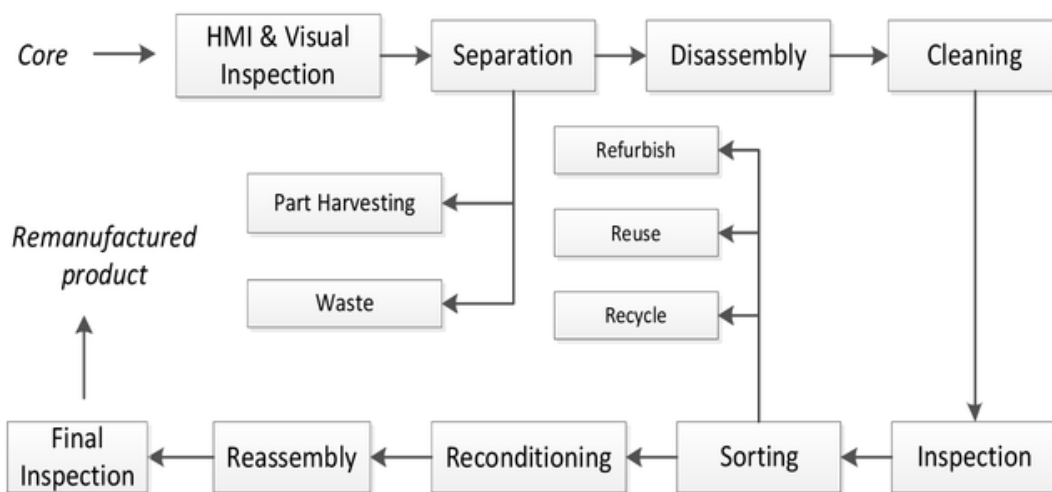
Fig. 3. Steps of mobile phone remanufacturing process.
