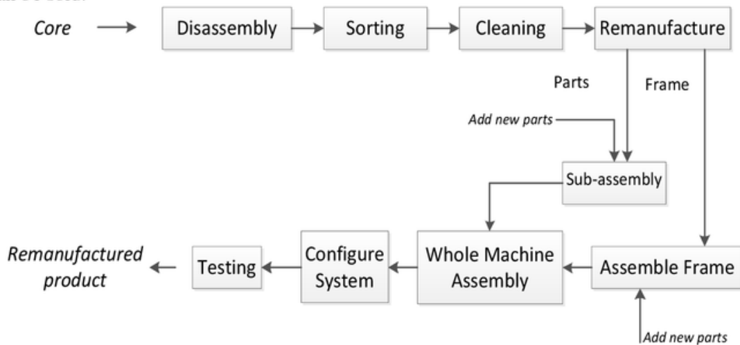
Fig. 2. Xerox remanufacturing process flow chart in Dundalk
