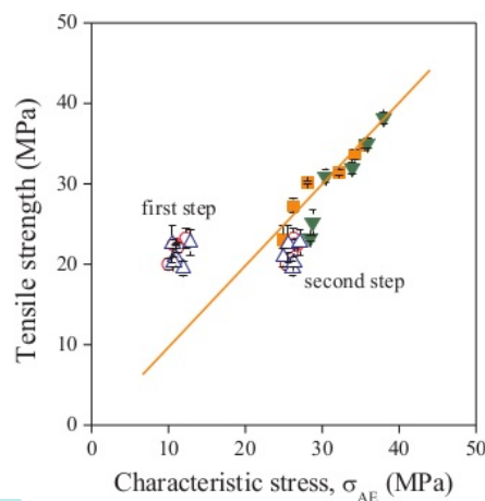
Fig. 12. Correlation between the tensile strength of the composites and the characteristic stresses determined by acoustic emission testing. Symbols are the same as in Fig. 1.
