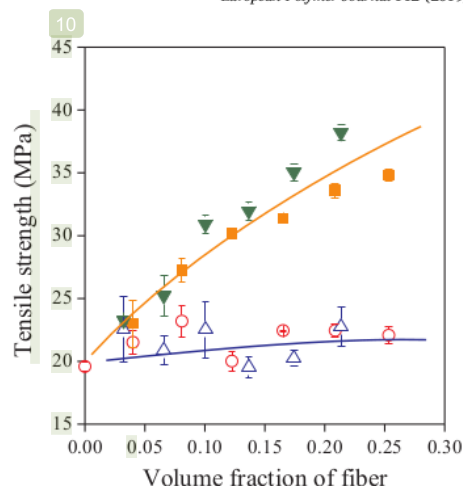
Fig. 3. Tensile strength of PP/lignocellulosic fiber composites plotted against fiber content. Symbols are the same as in Fig. 1.
