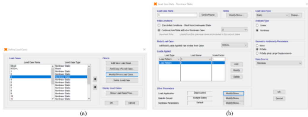
Figure 8. Loading history definition in SAP2000 (a) load case (b) nonlinear load case parameters
