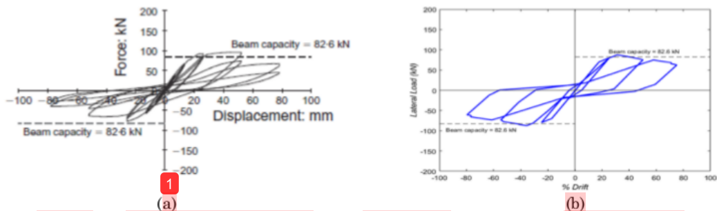
Figure 19. Comparison of hysteretic curve of specimen BSL-300 [33] (a) test (b) model
