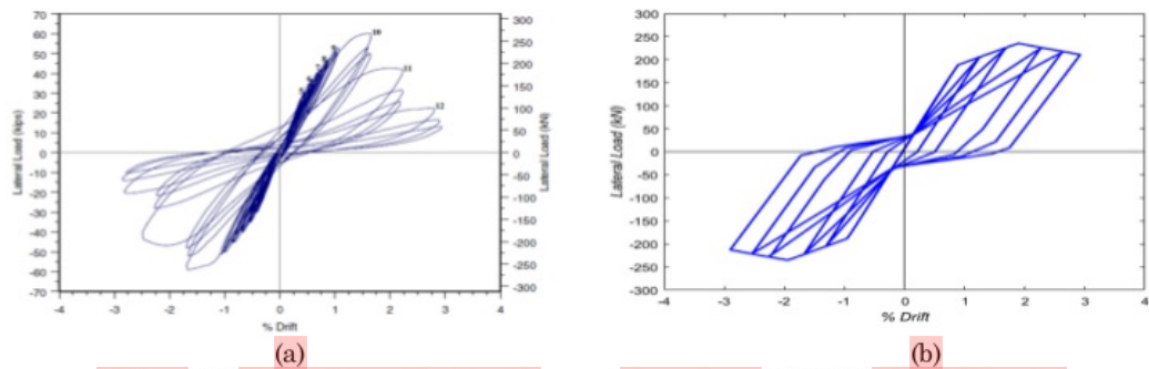
Figure 17. Comparison of hysteretic curve of specimen C5 [30] (a) test (b) model
