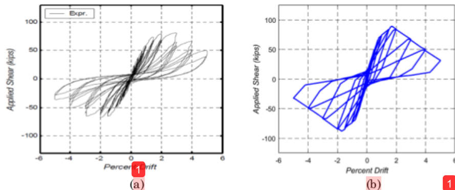
Figure 9. Comparison of hysteretic curves of specimen PEER-2250 [1] (a) test (b) model
