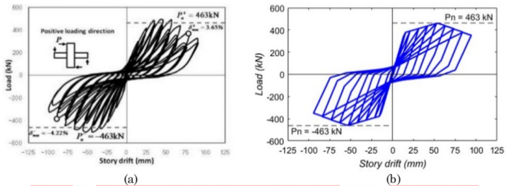
Figure 11. Comparison of hysteretic curves of specimen S1 [31] (a) test (b) model
