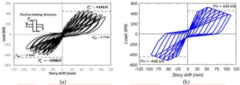
Figure 13. Comparison of hysteretic curve of specimen S3 [31] (a) test (b) model
