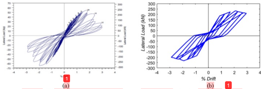
Figure 16. Comparison of hysteretic curve of specimen C2 [30] (a) test (b) model
