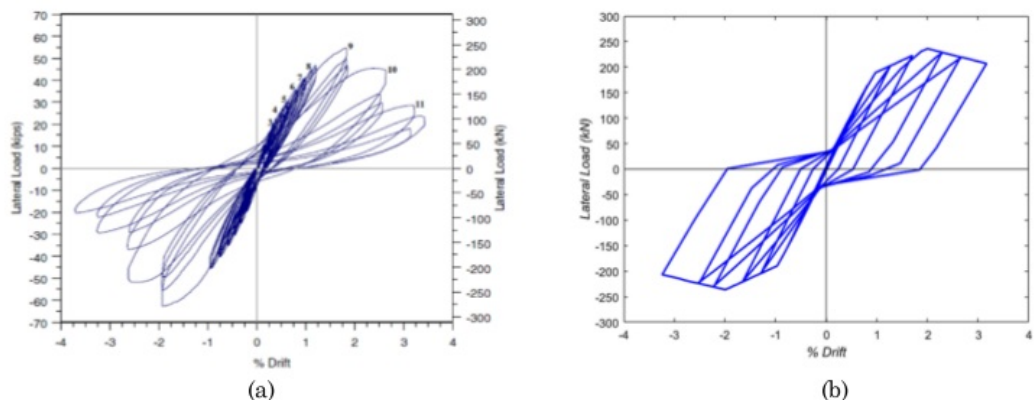
Figure 18. Comparison of hysteretic curve of specimen C6 [30] (a) test (b) model
