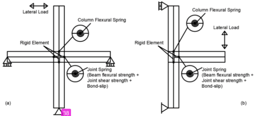
Figure 1. Proposed beam-column joint model for (a) internal joint and (b) external joint
