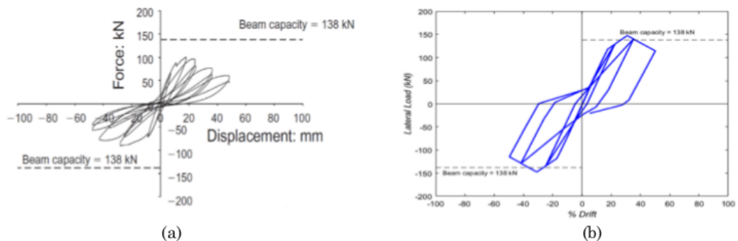
Figure 20. Comparison of hysteretic curve of specimen BSL-450 [33] (a) test (b) model
