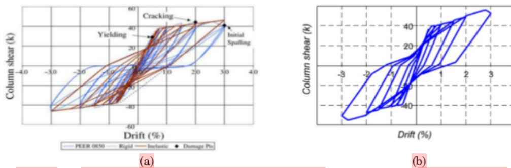
Figure 10. Comparison of hysteretic curves of specimen PEER-0850 [1] (a) test (b) model
