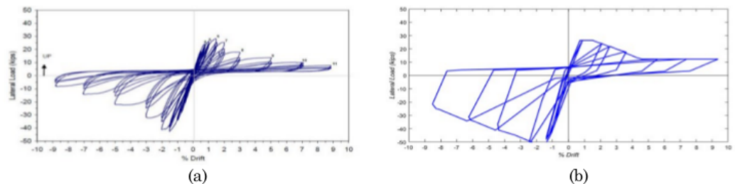
Figure 15. Comparison of hysteretic curve of specimen P2 [32] (a) test (b) model
