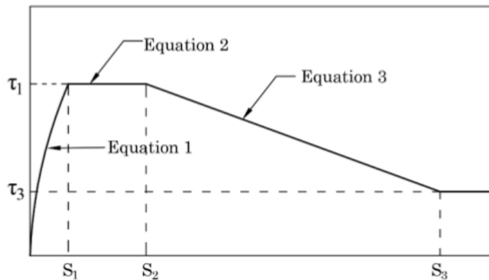
Figure 2. Monotonic envelope curve for bond-slip relationship (Elmorsi et al., 2000)
