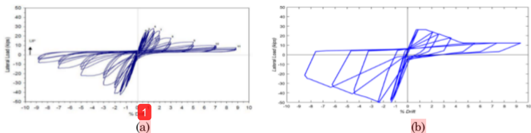
Figure 14. Comparison of hysteretic curve of specimen P1 [32] (a) test (b) model
