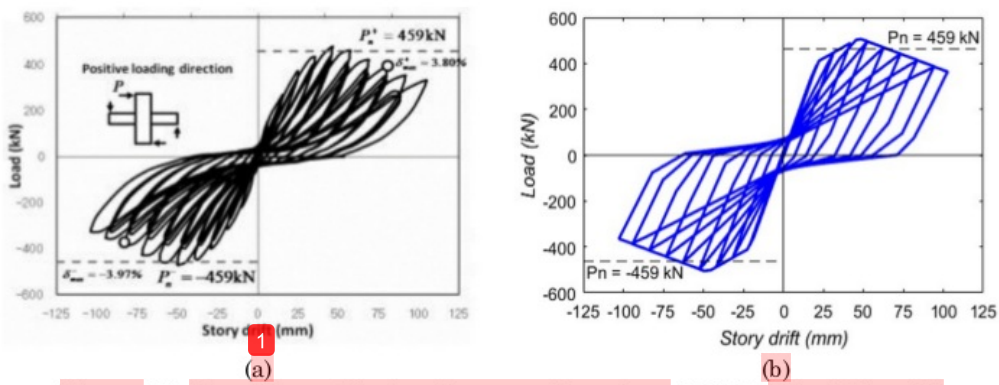
Figure 12. Comparison of hysteretic curves of specimen S2 [31] (a) test (b) model
