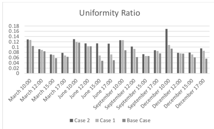
Figure 5. Average uniformity ratio Case 2, Case 1, and Base Case
