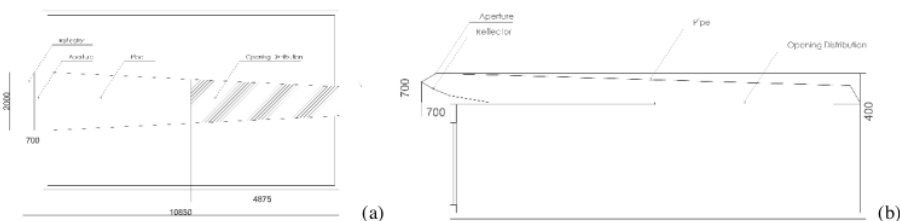
Figure 1. (a) Room plan with Light Pipe A system (b) Room section with Light Pipe A system
