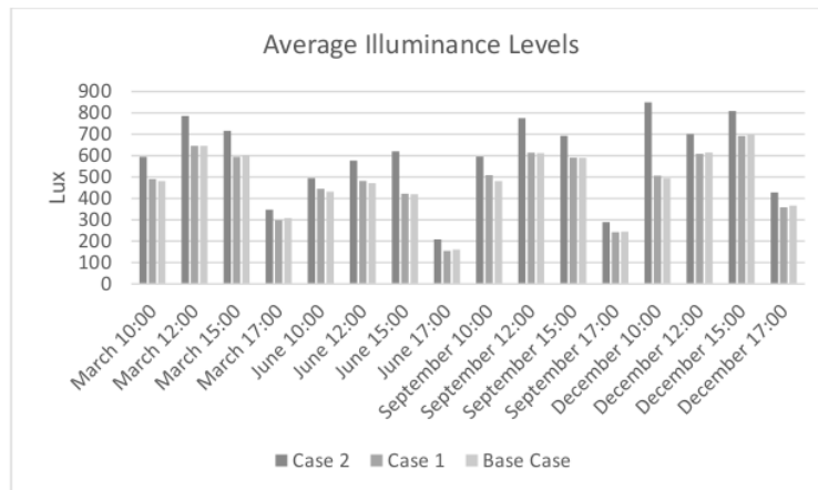
Figure 3. Average illuminance levels Case 2, Case 1, and Base Case
