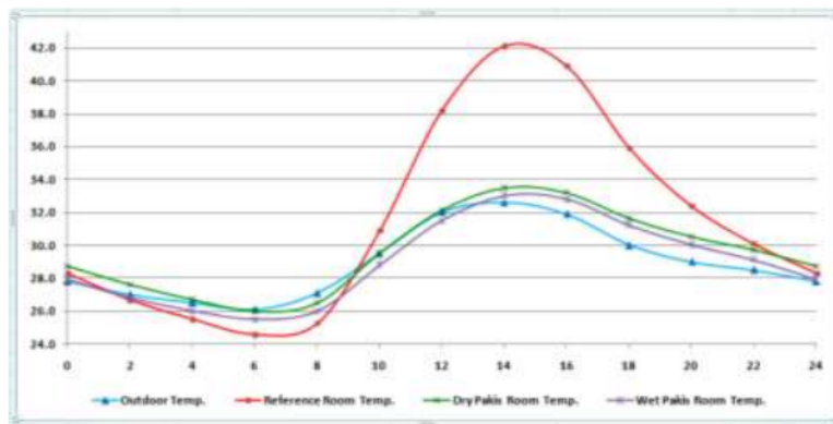
Figure 14 Room Temperatures on 3 models for September 2011
