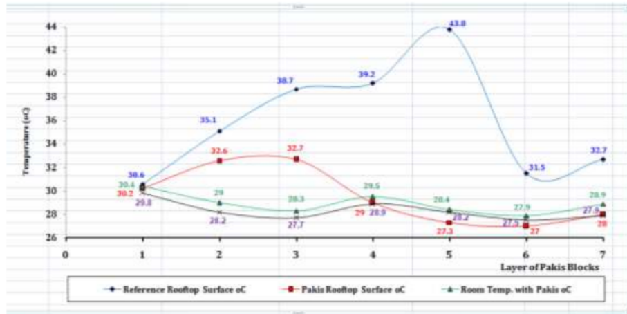
Figure 17 Thermal Performances of Pakis Thickness
