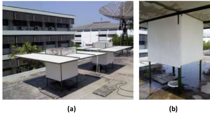
Figure 10. 1 meter length of horizontal shading device around the models (a), 4 sides of external walls covered with 2 cm foam (b)
