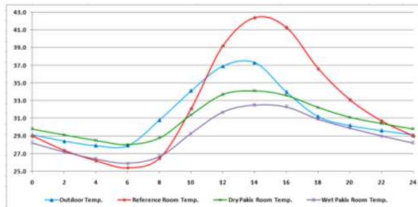
Figure 15 Room Temperatures on 3 models for October 2011
