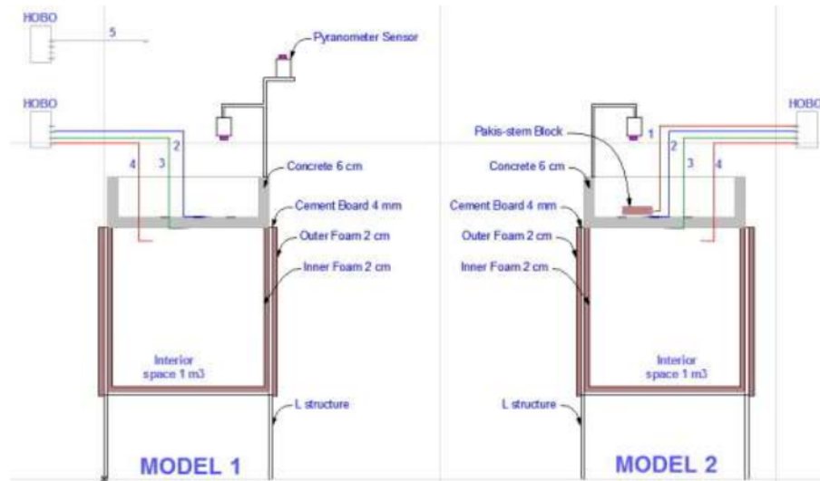
Figure 13 Diagram Processing on Models, Equipment and Procedures
