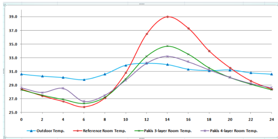
Figure 18 Room Temperatures on November 2011
