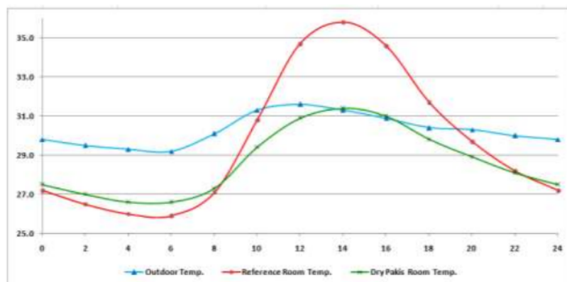
Figure 16 Room Temperatures on 3 models for November 2011
