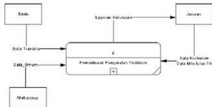
Gambar 2. Context Diagram
