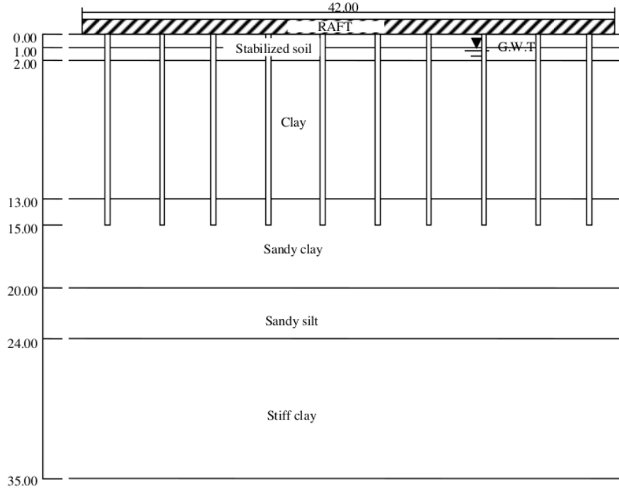
Figure 1: Geometry of model
