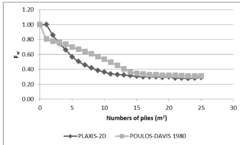
Figure 3: Settlement reduction factors considering numbers of piles
