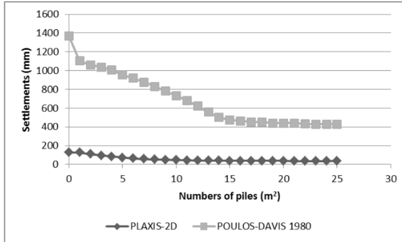
Figure 2: Settlements considering number of piles
