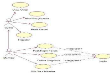
Gambar 2. Use Case Diagram Member dan Guest
