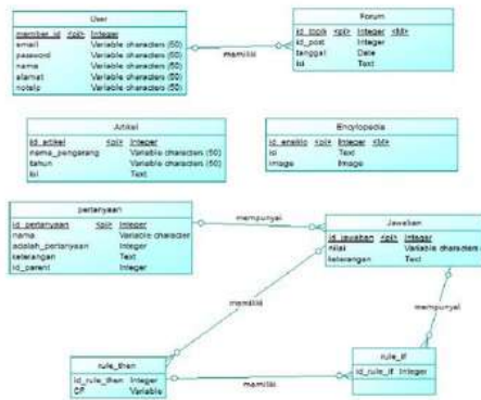
Gambar 3. Conceptual ERD
