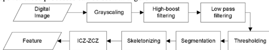
Figure 5. Digital image processing and feature extraction
