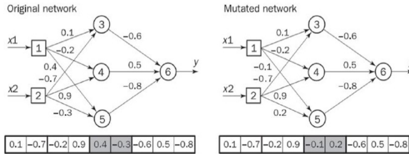
Figure 6. Mutation operation
