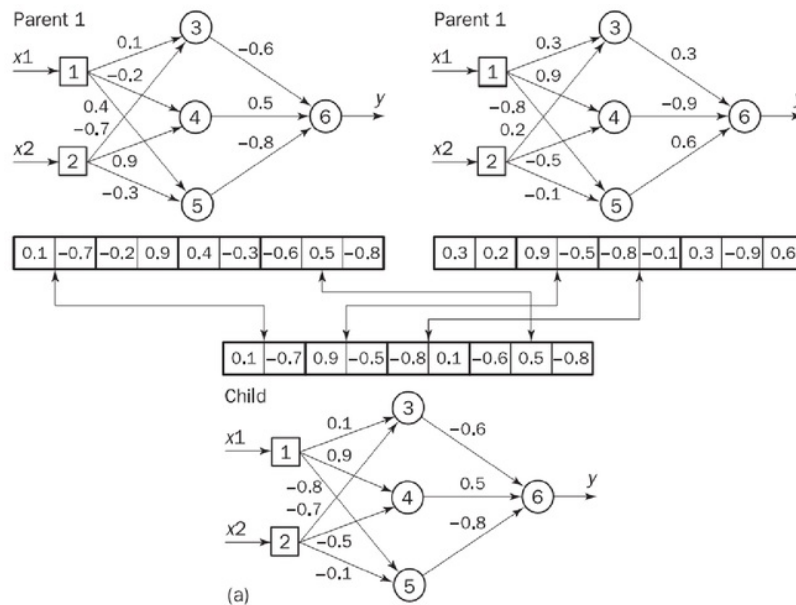
Figure 5. Crossover operation
