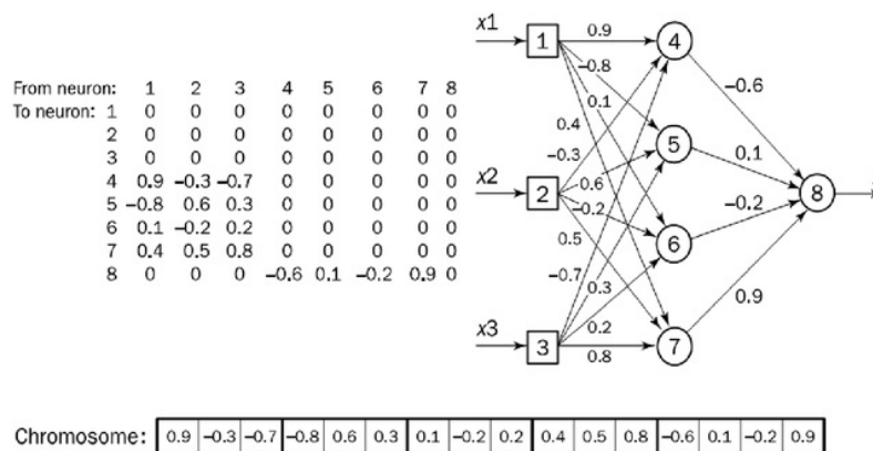
Figure 4. Encoding a network into a chromosome
