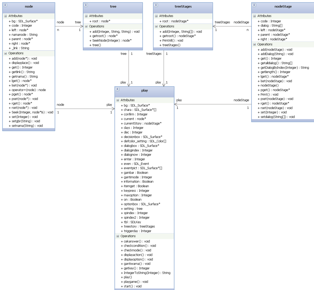
Gambar 5. Class Diagram Petualangan Timun Mas
