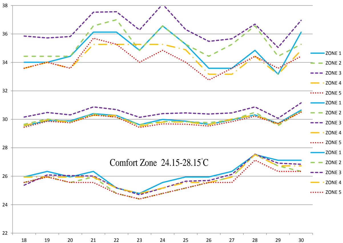
Figure 3. Temperature Profile of Field Measurement
