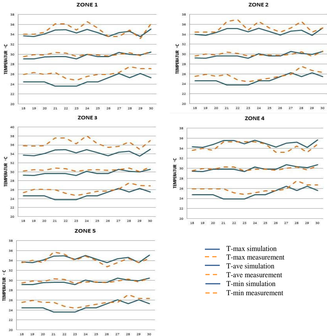
Figure 5. Validation air temperature of Steve tool simulation vs field measurement in each zone
