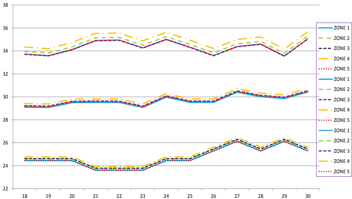
Figure 4. Temperature profile of STEVE tool Simulation
