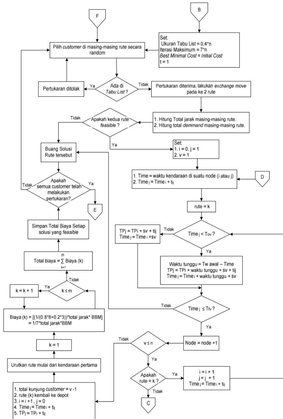
Gambar 2. Flowchart Algoritma Tabu Search
