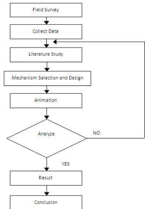
Figure 4. Research methodology
