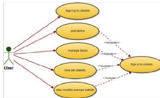
Fig 2. Use Case Diagram for Apps
