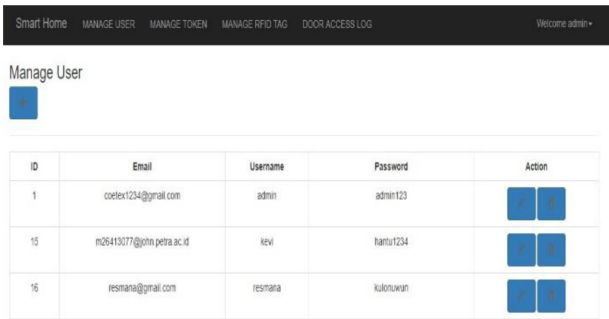
Fig. 8. The User Management page.
