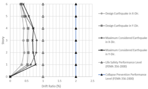
Figure 7. Drift Ratios of Hotel X due to Design and Maximum Considered Earthquake Compared to FEMA 356-2000 limits
