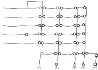
Figure 14. Frame D Plastic Hinges due to Maximum Considered Earthquake in y-direction
