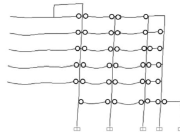
Figure 12. Frame D Plastic Hinges due to Design Earthquake in y-direction
