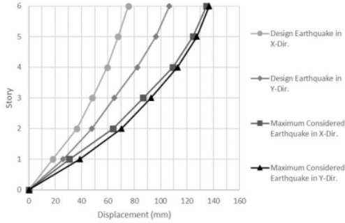
Figure 6. Hotel X Displacement Graph
