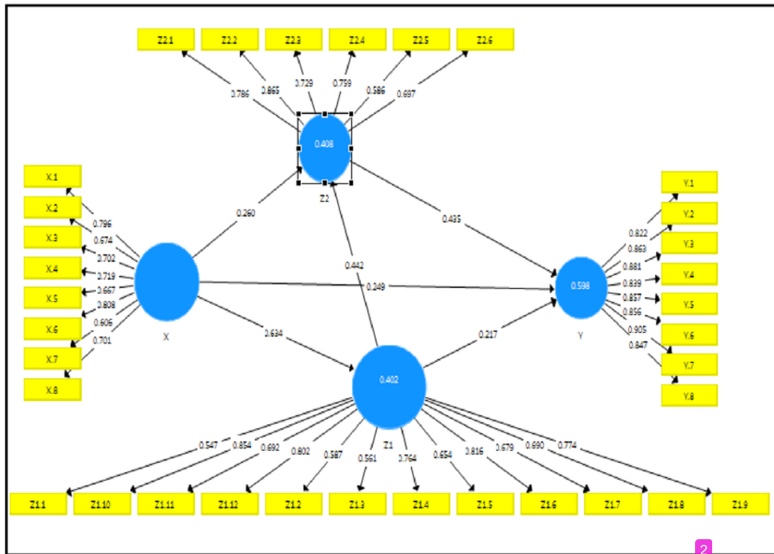
Picture-2: PLS Model
