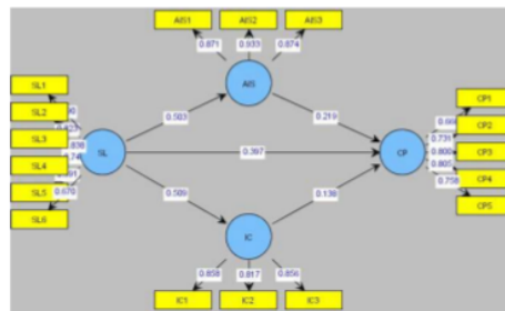
FIGURE 2 PLS OUTPUT
