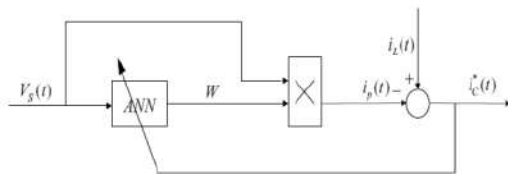
Gambar 3. Perhitungan Bobot Jaringan Saraf Tiruan
