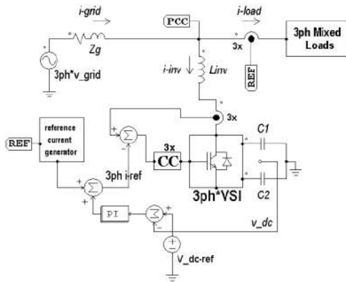
Gambar 1. Konfigurasi Shunt Active Power Filter
