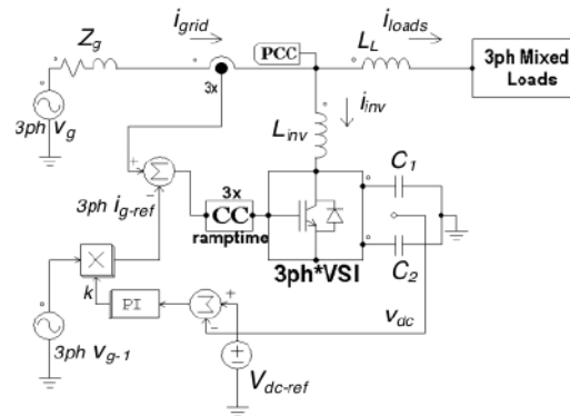
Figure 2. The shunt APF configuration
