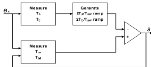
Figure 5. The functional block diagram of PRCC
