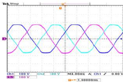
Figure 8. The grid voltages
