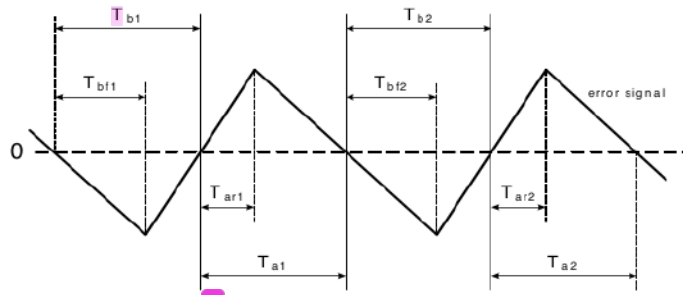
Figure 3. Current error signal
