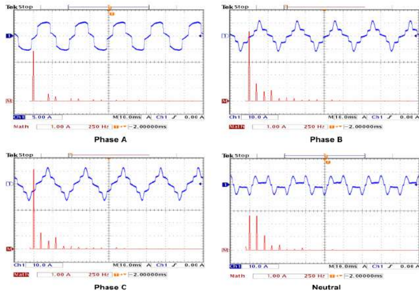
Figure 9. Phase and neutral currents for mixed loads
