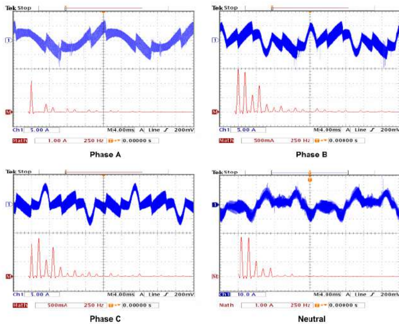
Figure 12. Phase and neutral currents of the CC-VSI
