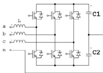
Figure 1. Three-phase Voltage Source Inverter (VSI)
