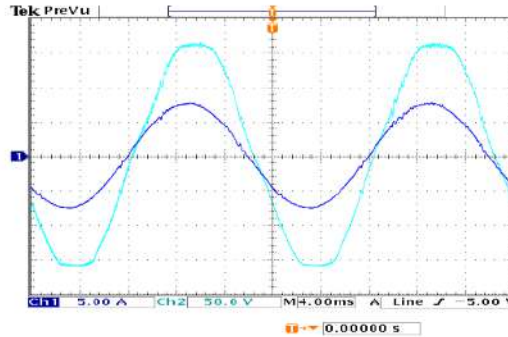
Figure 11. Phase-A grid voltage and current after compensation
