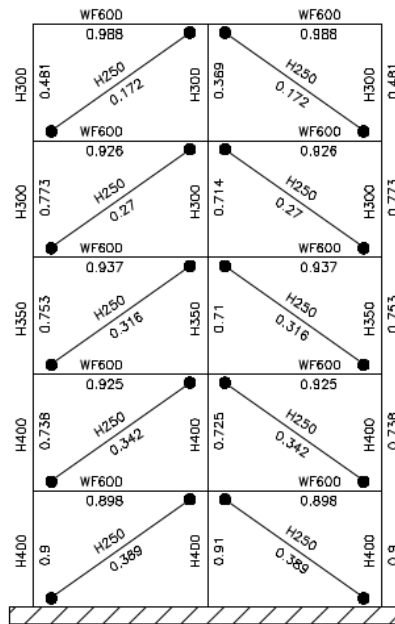
Figure 11: Steel Design Result.
