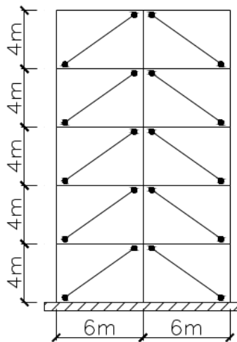
Figure 10: The Structure Considered.
