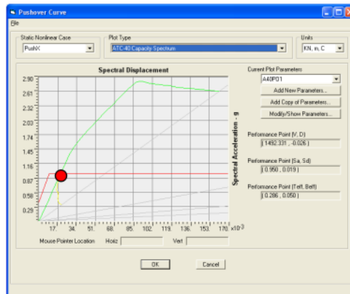
Figure 12: Performance Point
