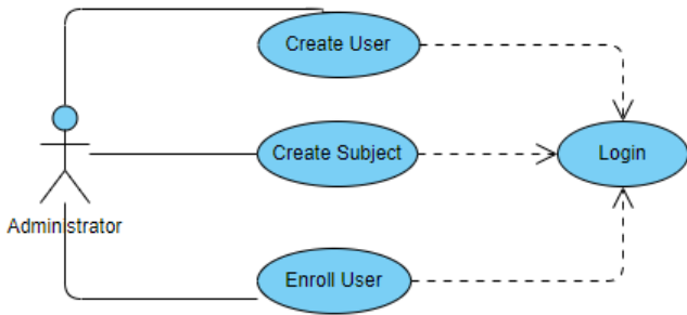
Fig. 2. Use case diagram of Administrator
