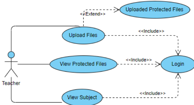
Fig. 3. Use case diagram of teacher
