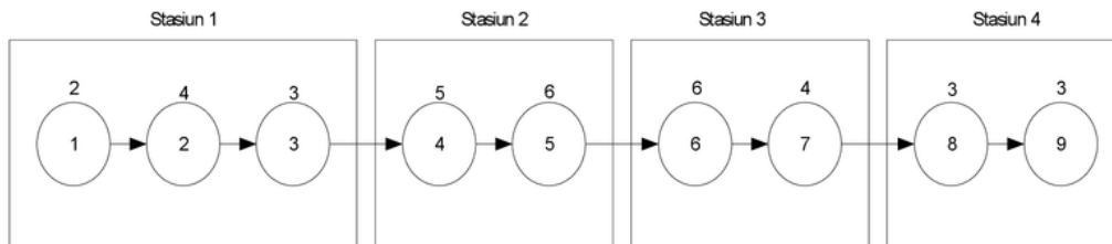
Gambar 1. Keseimbangan lintasan straight line
