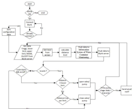
Figure 3 Flowchart
