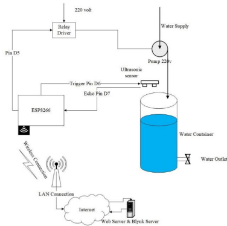
Figure 1 Hardware System
