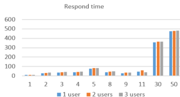
Figure 8. Respond time chart.
