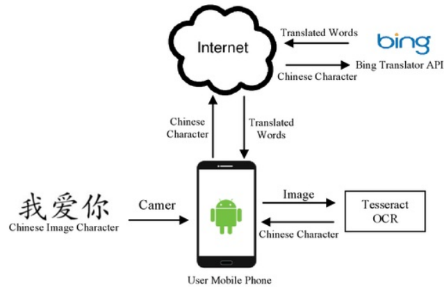
Fig 2: Chinese Character Translator
