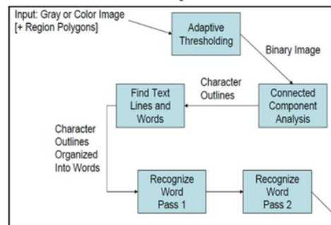
Fig 1: Tesseract Architecture [5].
