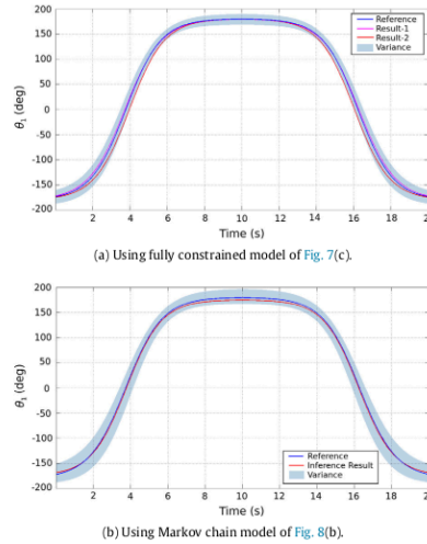
Fig. 14. The inverse kinematics results for \theta_1 . For the other joints, the results were very similar.
