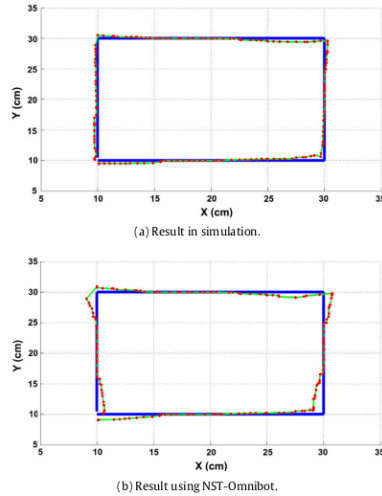
Fig. 15. (a) The inference result of kinematic models in a simulation environment. The outputs of the inverse kinematics network shown in Fig. 7(c) were sent to the forward kinematics network shown in Fig. 7(c). The blue line is the trajectory for the robot to follow and the red dots connected by the green line is the resulting trajectory. (b) The experiment was conducted using the real robot. (For interpretation of the references to color in this figure legend, the reader is referred to the web version of this article.)
