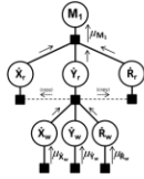
Fig. 6. An inverse kinematics model as a result of decoupling the network shown in Fig. 5c by exploiting independences given the observed variables. \mu_{M_1} , \mu_{X_c} , \mu_{Y_c} , and \mu_{R_c} are messages representing “beliefs” about variable’s values propagating through the network. Thin arrows indicate the flow of messages during belief propagation to produce final output at the “root” node ( M_1 ).
