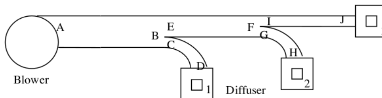
Gambar 1. Layout model
