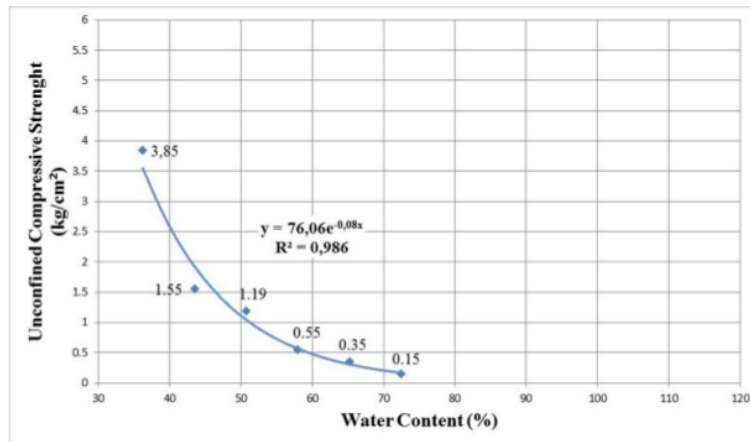
Figure 3. Changes in unconfined compressive strength due to water content variation at Makarya.
