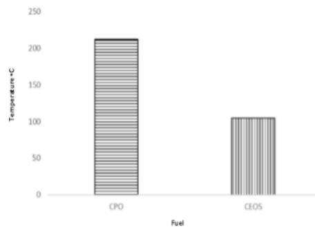
Figure 3: Comparison of flash point between CPO and CEO5
