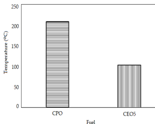
Figure 3. Flash point comparison of CPO and CEO5
