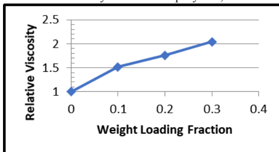
Fig. 8. Relative viscosity vs. weight loading fraction at 210 °C at the shear rate of 500 ( 1\text{ s}^{-1} )
