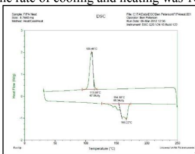
Fig. 4. DSC results for neat polypropylene co-polymer.
