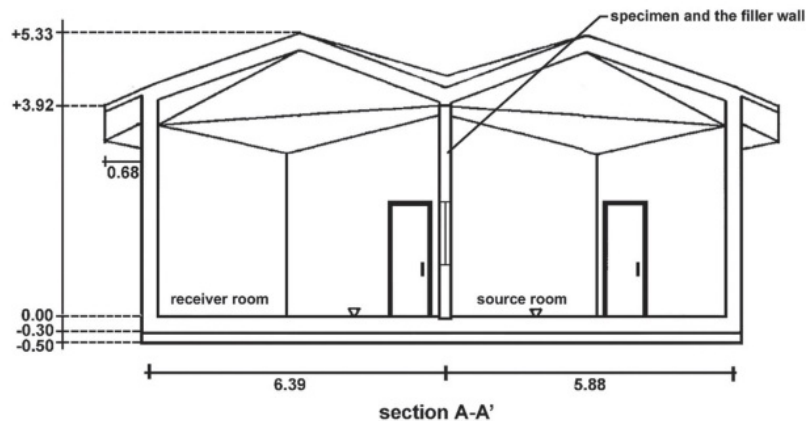
Figure 6. The A-A' section of the testing rooms.
