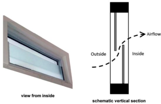
Figure 3. A typical fixed open glass window used in Indonesia, usually for bathrooms or other small rooms.
