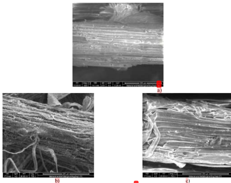
FIGURE 2. SEM micrographs of a) untreated bagasse fibers, b) \text{Ca(OH)}_2 treated bagasse fibers, and c) NaOH treated bagasse fibers.
