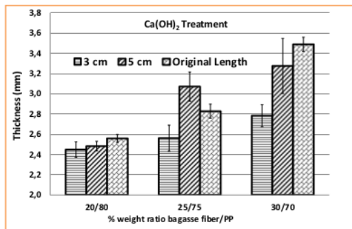
FIGURE 3. Composite thickness against bagasse fiber length and wt. % ratio of bagasse fiber/PP (treated with \text{Ca}(\text{OH})_2 )
