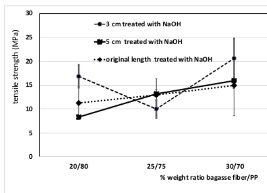
FIGURE 6. Tensile strength of composite samples using different fiber length and % wt. ratio of bagasse fiber/PP (treated with NaOH)
