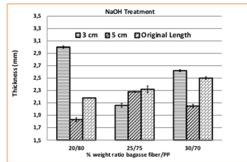
FIGURE 4. Composite thickness against bagasse fiber length and wt. % ratio of bagasse fiber/PP (treated with \text{NaOH} )
