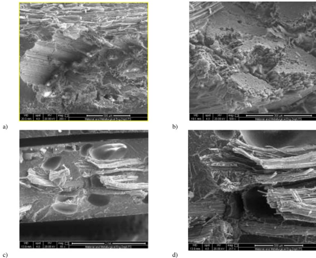
FIGURE 7. SEM micrographs of fracture surface of tensile test samples of a), b) composites with 20/80 wt% bagasse fibers/PP with fiber length of 5 cm and treated with \text{Ca(OH)}_2 and c), d) composites with 25/75 wt% bagasse fibers/PP with fiber length of 3 cm and treated with NaOH
