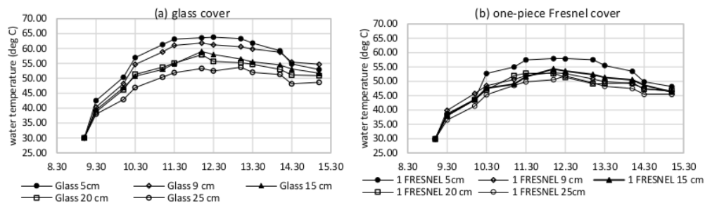
Figure 3. The effect of air gap for glass cover and one-piece Fresnel lens cover on water temperature.
