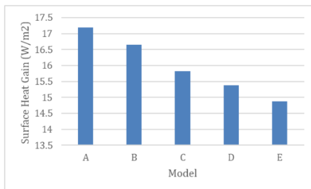
Figure 5. Solar incident radiation on second skin façade
