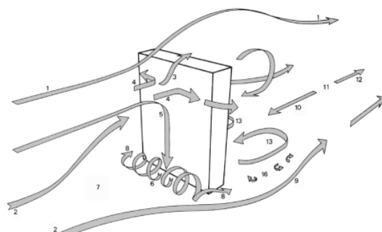
Figure 1. Wind flow pattern around a high-rise building [9]
