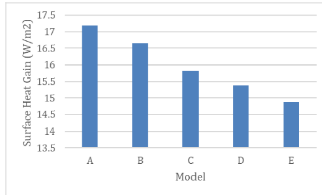
Figure 5. Solar incident radiation on second skin façade
