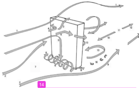
Figure 1. Wind flow pattern around a high-rise building [9]
