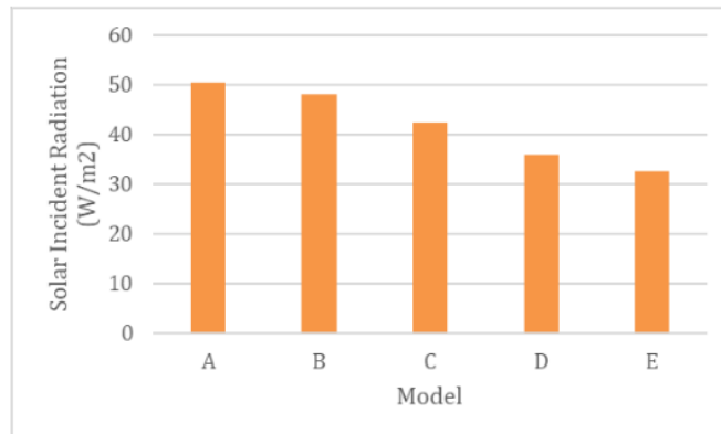
Figure 6. Surface heat gain on the east façade
